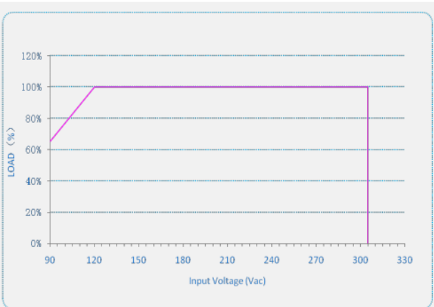
Output Power Vs. Input Voltage
